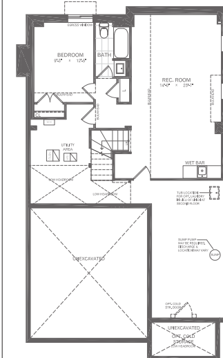
Opt. Finished Basement - Elevation A
