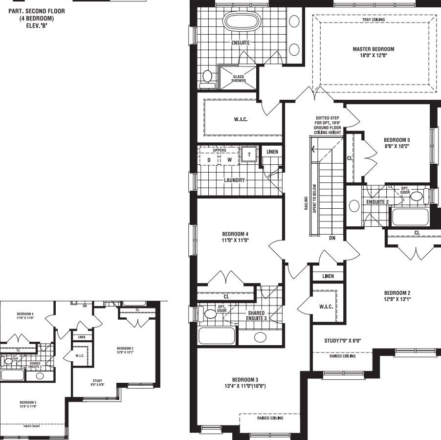
OPT. SECOND FLOOR (4 BEDROOM) ELEV. A'
