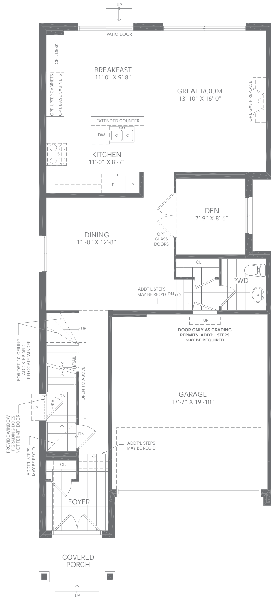
GROUND FLOOR PLAN B
