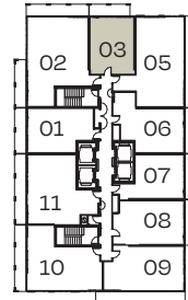
LEVEL 06-09, 25-29
